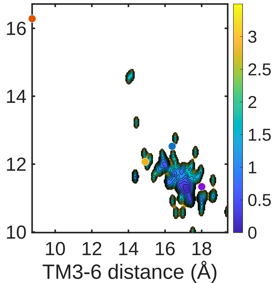
Cluster C3
