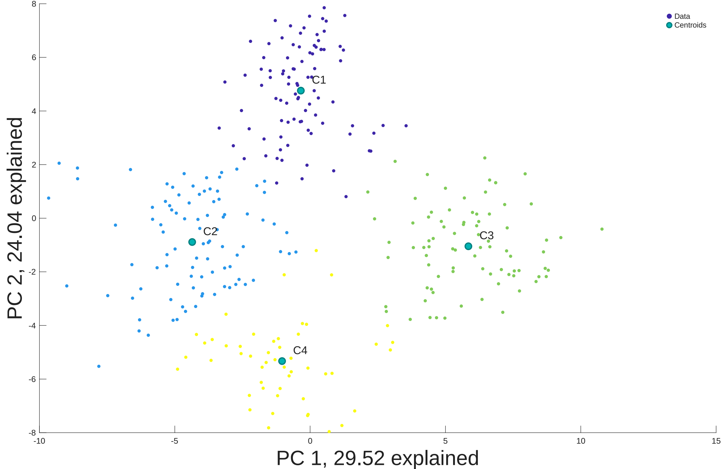
Clustering with 2 PCs, 53.56 explained total
