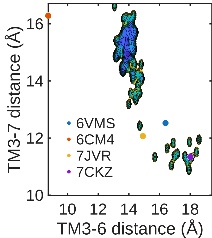
Cluster C1
