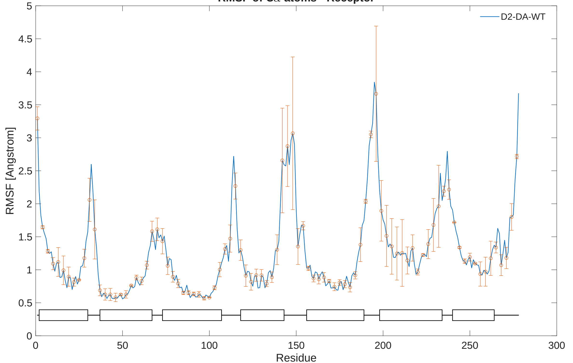
RMSF of C \alpha atoms - Receptor
