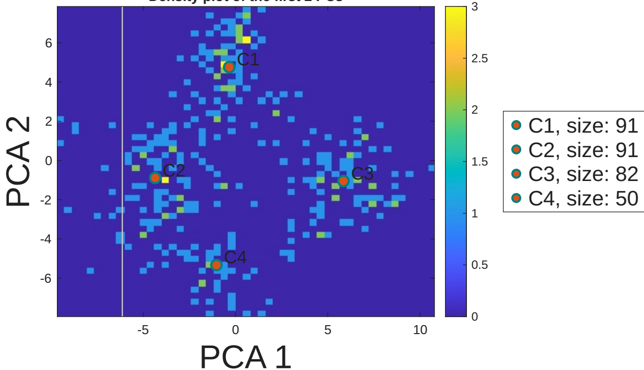
Density plot of the first 2 PCs
