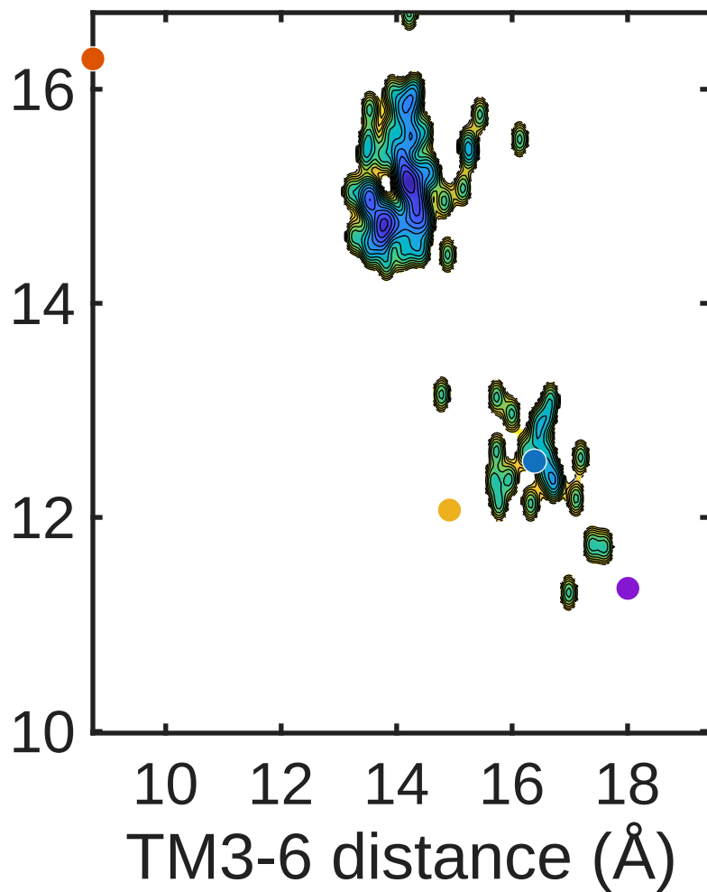
Cluster C2
