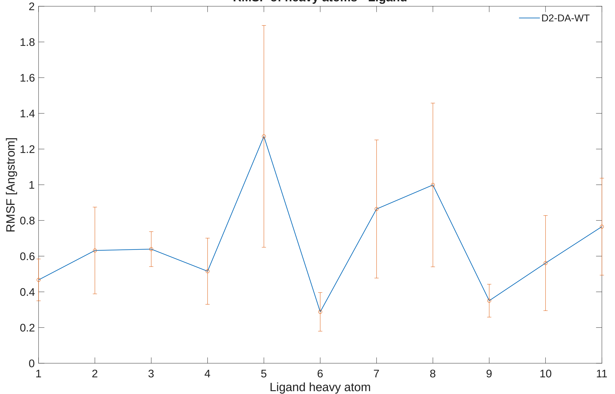
RMSF of heavy atoms - Ligand
