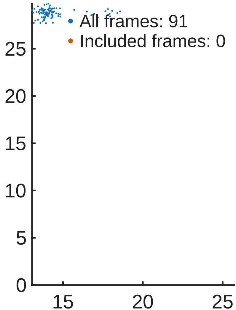
Cluster C1
