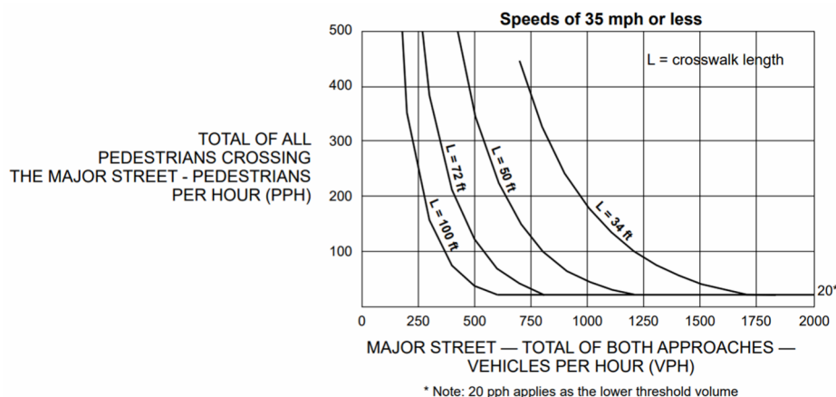
Figure 3. MUTCD Figure 4J-1 for the installation of PHBs on roadways with speeds of 35 mph or less
