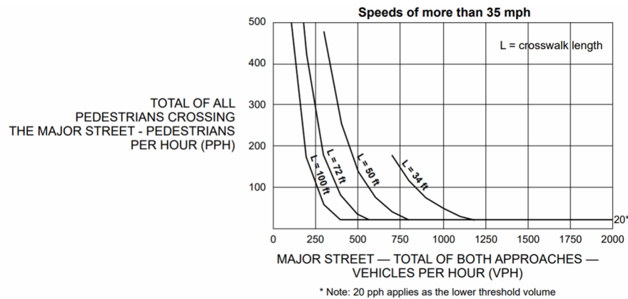
Figure 4. MUTCD Figure 4J-2 for the installation of PHBs on roadways with speeds of more than 35 mph
