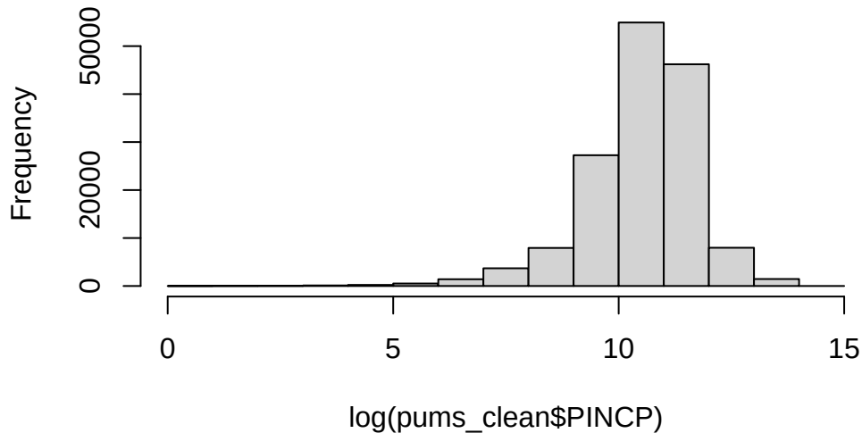
Histogram of \log(\text{pums\_clean}\$PINCP)
