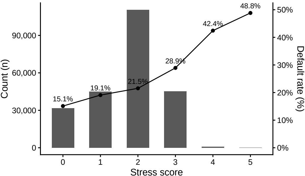
Default rate rises with stress score
