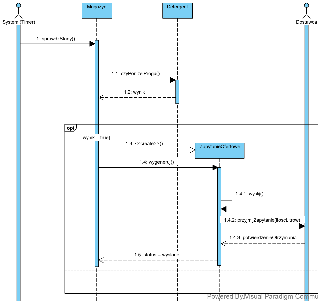
sd [Sequence Diagram3]
