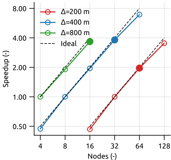
a) Strong scaling: speedup
