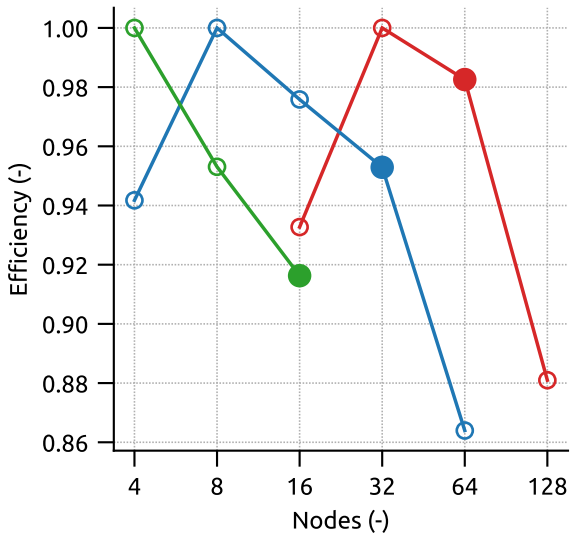
b) Strong scaling: efficiency
