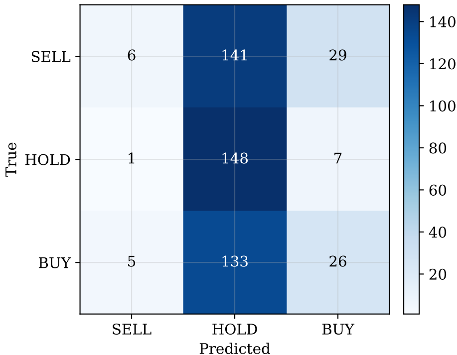
Confusion matrix (test, SWA model)
