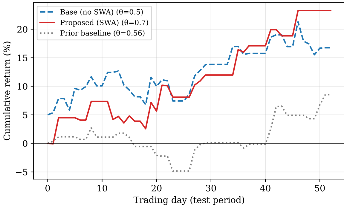
Out-of-sample equity curves (test set)
