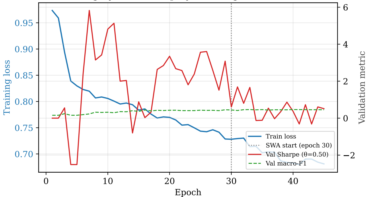
Training dynamics (deployed configuration, seed 2)
