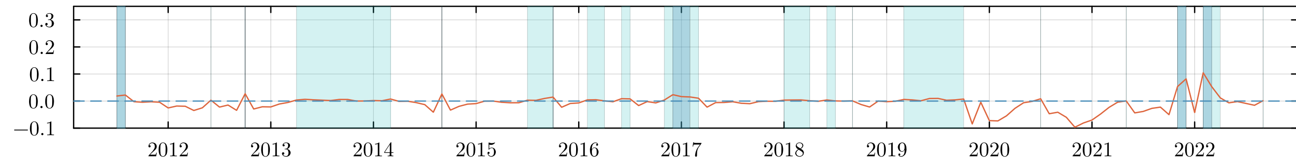
TV-EWD vs. AR
