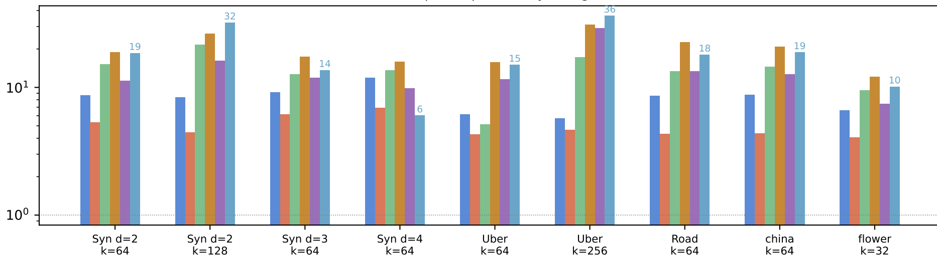
Reduction in distance computations over Lloyd's algorithm
