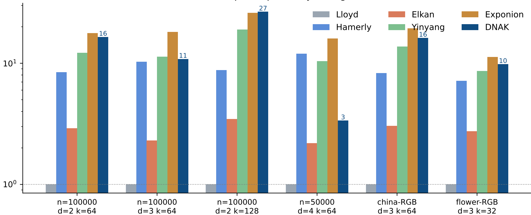
Wall-clock speedup vs Lloyd's algorithm
