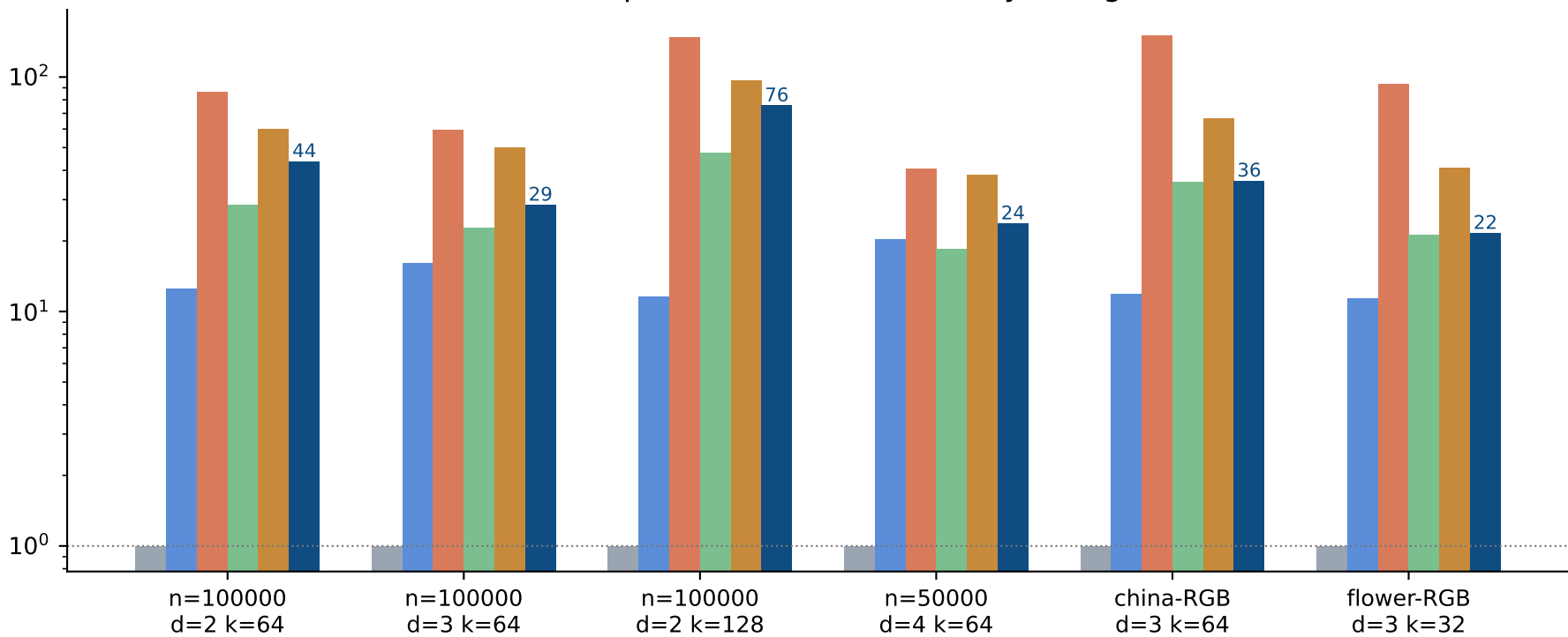
Distance-computation reduction vs Lloyd's algorithm
