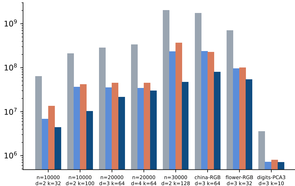
Total operations (distances + bound maintenance)
