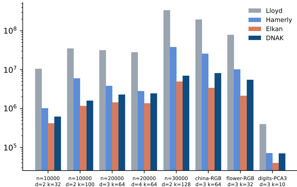
Point-centroid distance computations
