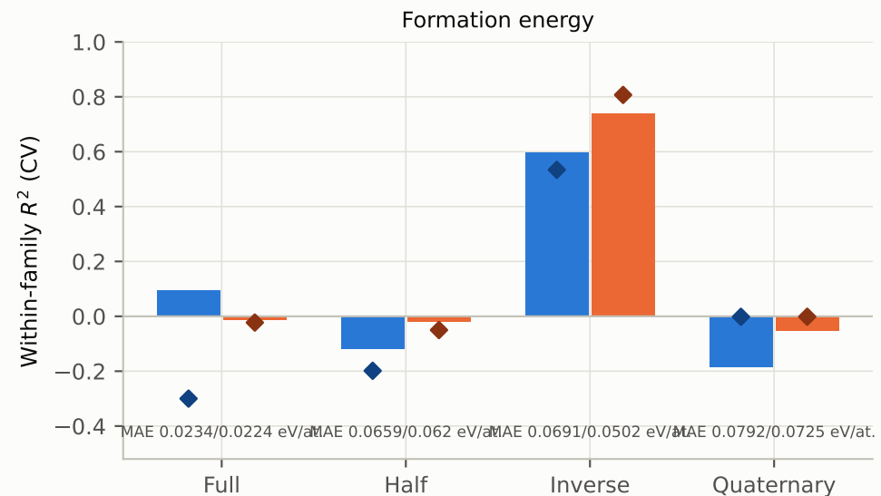
Per-family breakdown: pooled vs family-specific models (bars clipped at -0.3; MAE shown pooled/family)
