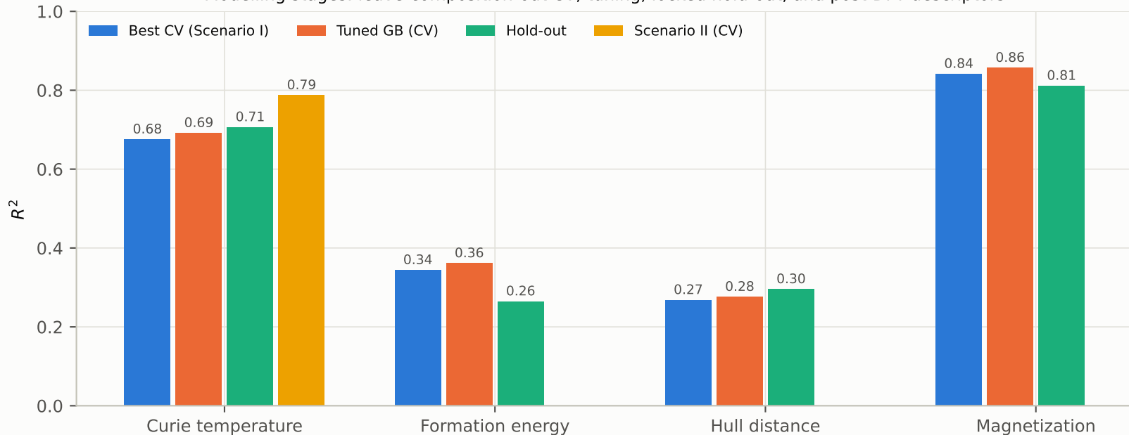
Modelling stages: leave-composition-out CV, tuning, locked hold-out, and post-DFT descriptors
