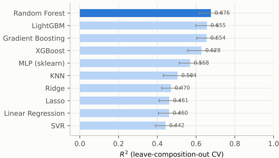
Curie temperature (MAE best = 108 K)
