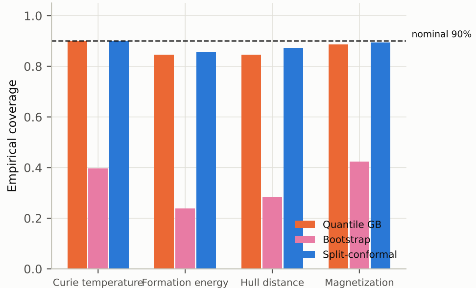
(b) Coverage of nominal 90% intervals
