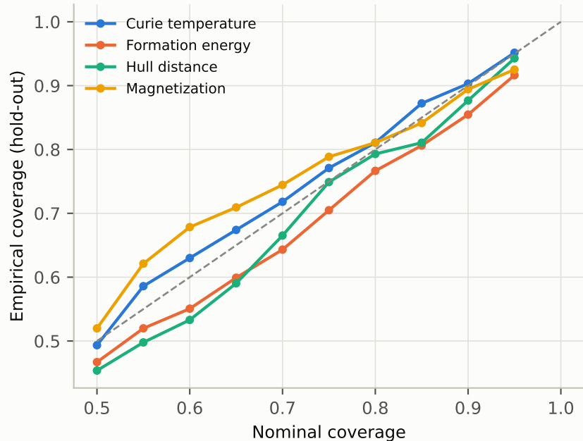
(a) Split-conformal reliability
