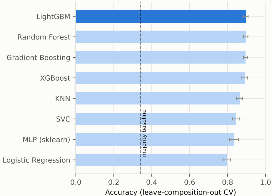
(a) Heusler-type classification, Tier A descriptors only
