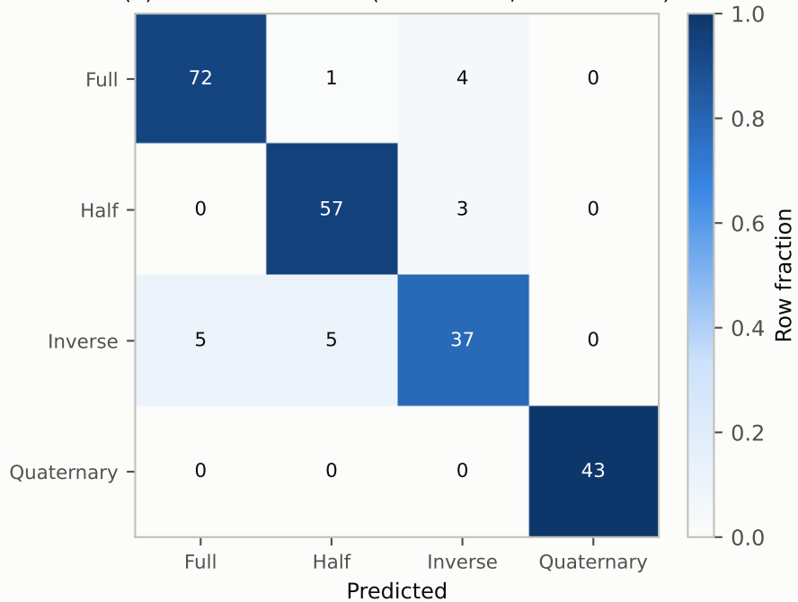
(b) Hold-out confusion (acc = 0.921, AUC = 0.985)
