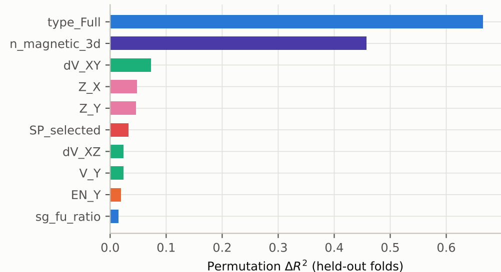
Hull distance
