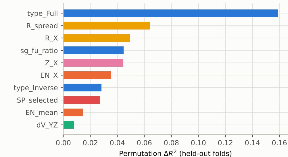
Hull distance
