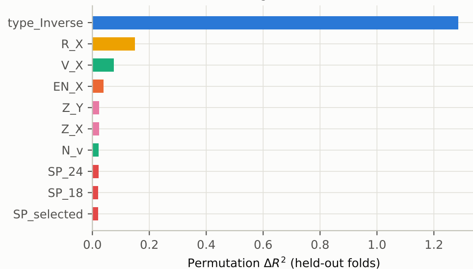
Magnetization
