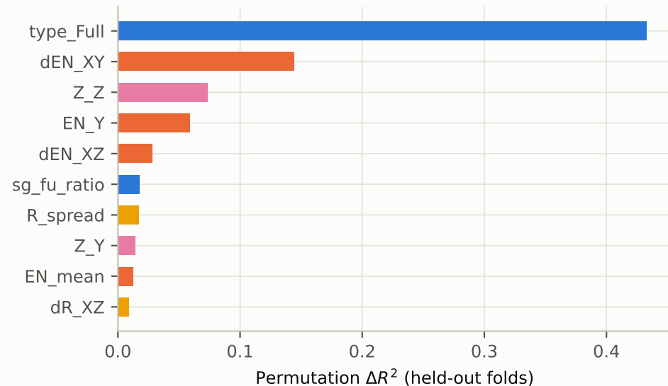
Magnetization
