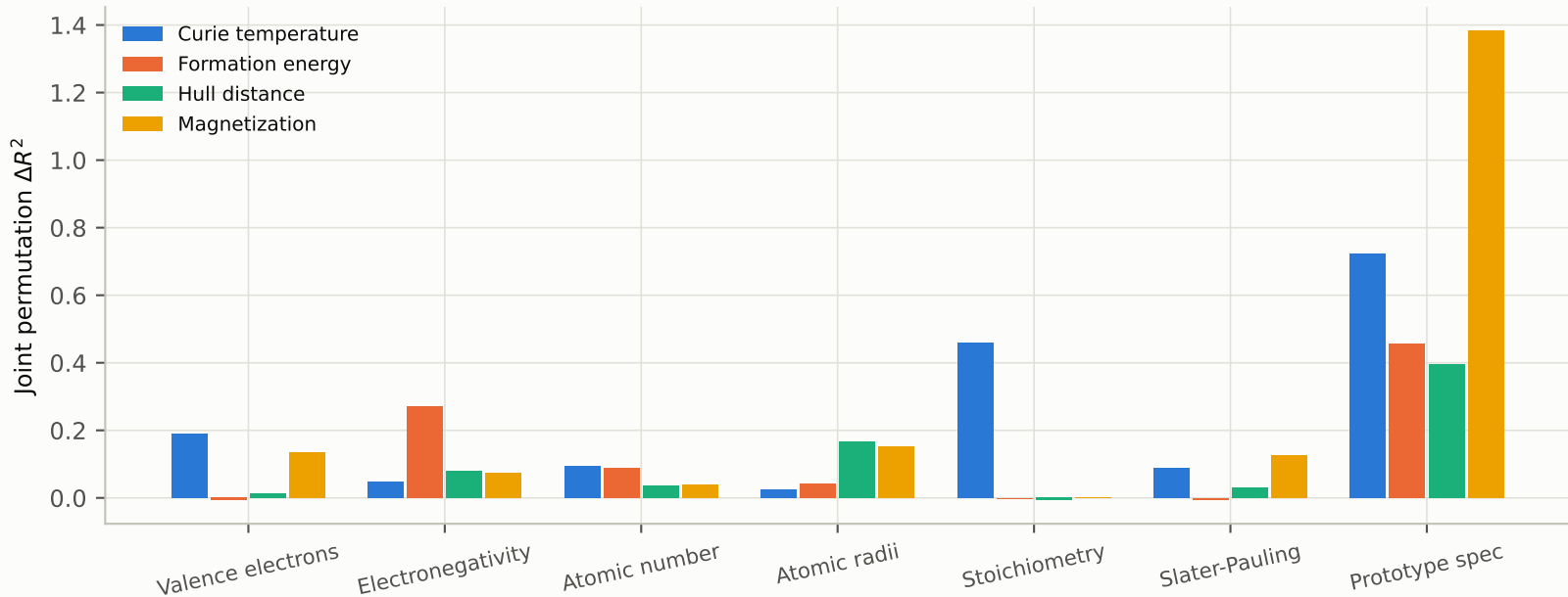
Collinearity-robust block importance (descriptor families permuted jointly)
