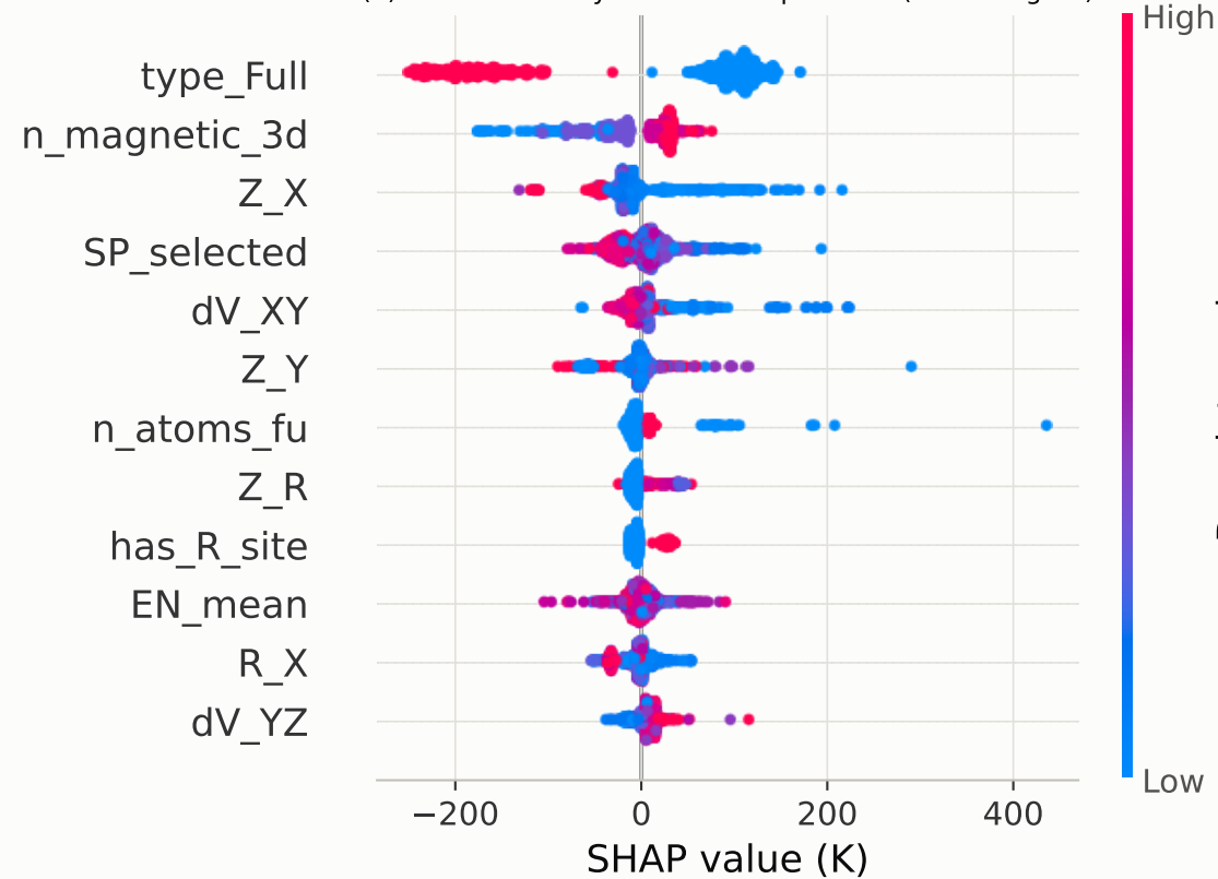
(a) SHAP summary — Curie temperature (GB surrogate)
