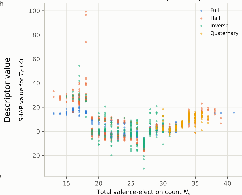
(b) SHAP dependence on N_v by Heusler type
