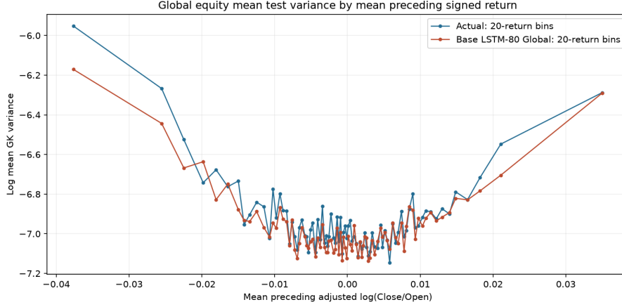
Figure 6.24: Global equity date-level mean adjusted Garman–Klass variance (blue) and saved Base LSTM-80 Global forecast (red) against the mean preceding signed adjusted open-to-close log return on 1,760 test dates, averaged across 88 bins of 20 dates.
