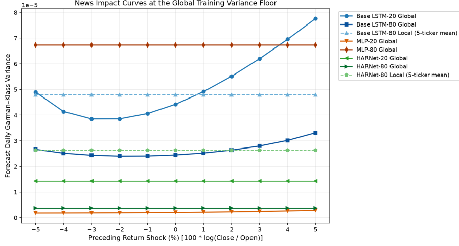
Figure 6.25: One-step forecast daily adjusted Garman–Klass variance against the synthetic signed return shock for eight MCS variants; the two RFSV variants are omitted.
