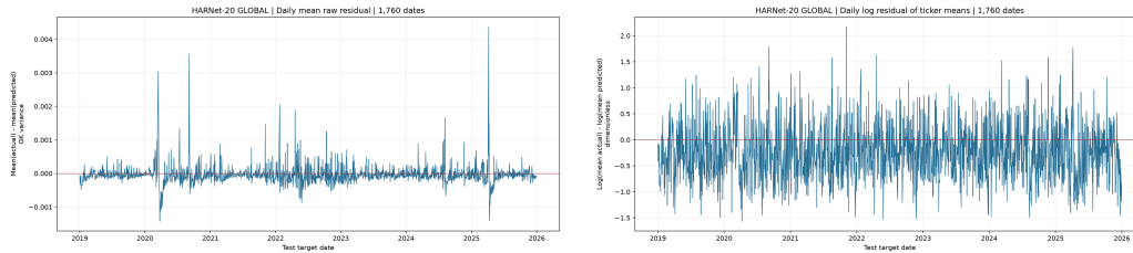
Figure 6.9: HARNet-20 Global: raw and log daily cross-ticker mean residual timelines (left and right).
