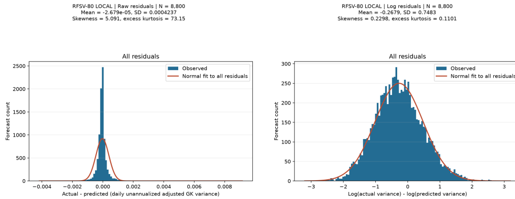
Figure 6.22: RFSV-80 Local: raw and log individual-residual histograms (left and right).
