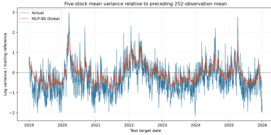
Figure 6.26: Natural log ratio of the five-stock mean observed (blue) or MLP-80 Global forecast (red) daily adjusted Garman–Klass variance to the mean of the five stock-specific preceding 252-observation rolling references, on 1,760 shared 2019–2025 test dates.
