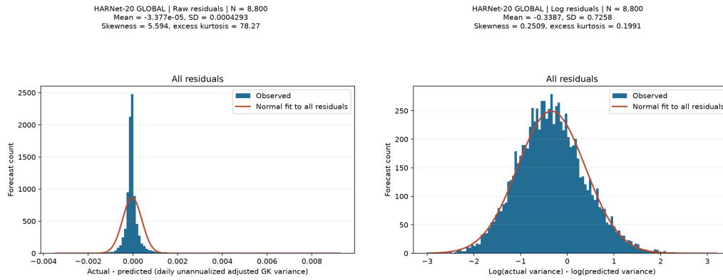
Figure 6.10: HARNet-20 Global: raw and log individual-residual histograms (left and right).
