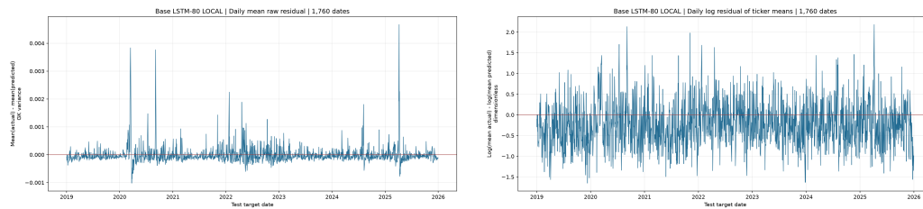
Figure 6.7: Base LSTM-80 Local: raw and log daily cross-ticker mean residual timelines (left and right).
