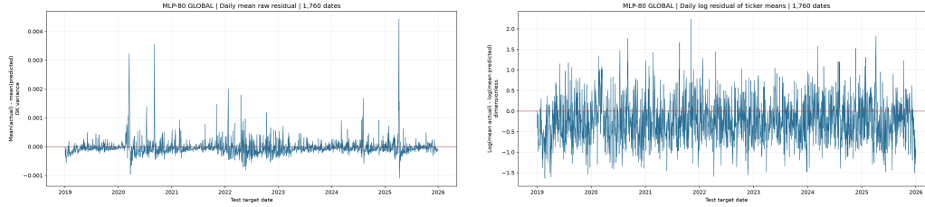
Figure 6.17: MLP-80 Global: raw and log daily cross-ticker mean residual timelines (left and right).
