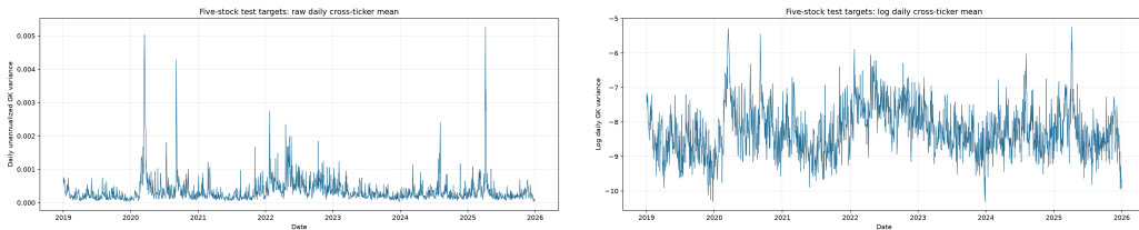
Figure 6.1: Five-stock test targets: daily mean unannualized adjusted Garman–Klass variance (left) and its natural logarithm (right).
