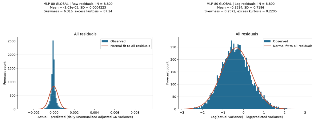
Figure 6.18: MLP-80 Global: raw and log individual-residual histograms (left and right).
