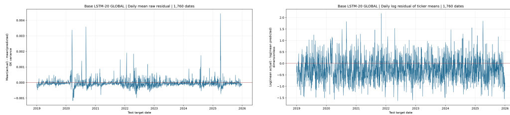
Figure 6.3: Base LSTM-20 Global: raw and log daily cross-ticker mean residual timelines (left and right).
