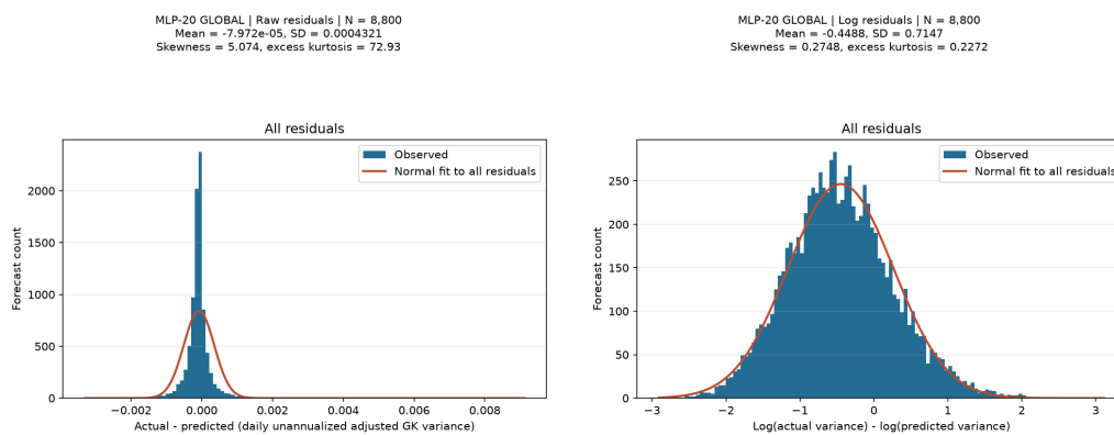
Figure 6.16: MLP-20 Global: raw and log individual-residual histograms (left and right).
