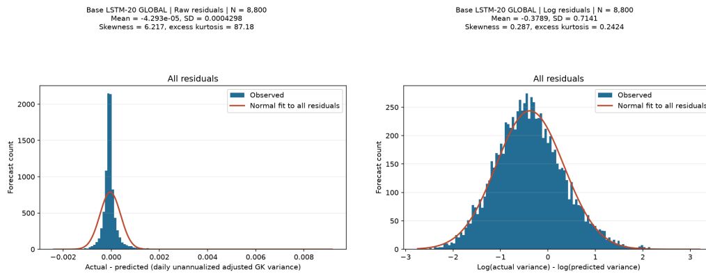
Figure 6.4: Base LSTM-20 Global: raw and log individual-residual histograms (left and right).
