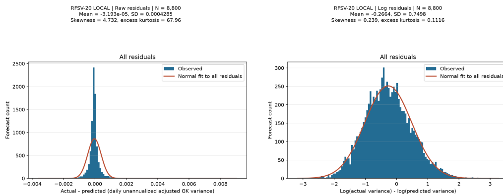
Figure 6.20: RFSV-20 Local: raw and log individual-residual histograms (left and right).
