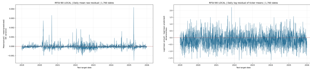
Figure 6.21: RFSV-80 Local: raw and log daily cross-ticker mean residual timelines (left and right).
