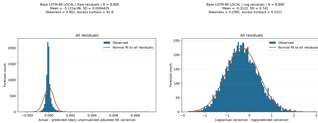
Figure 6.8: Base LSTM-80 Local: raw and log individual-residual histograms (left and right).
