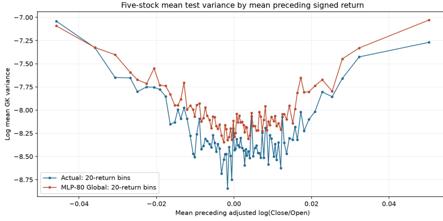
Figure 6.23: Log five-stock mean observed (blue) and MLP-80 Global forecast (red) daily adjusted Garman–Klass variance against mean preceding signed adjusted open-to-close log return, averaged across 88 consecutive bins of 20 return-sorted test dates.
