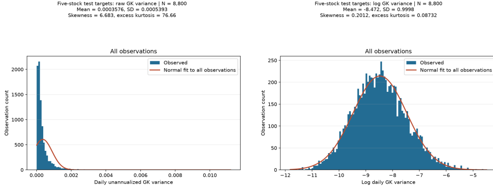
Figure 6.2: Five-stock test targets: pooled raw and log variance histograms (left and right). Each shows all 8,800 targets; the orange curve is a full-sample normal fit.
