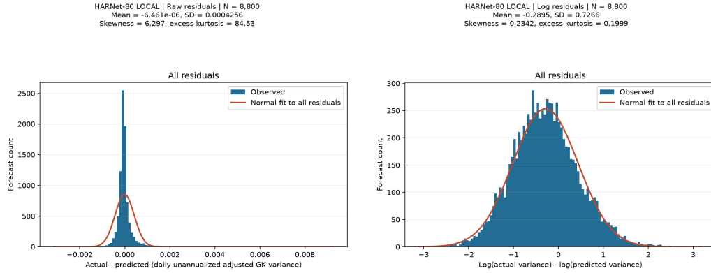
Figure 6.14: HARNet-80 Local: raw and log individual-residual histograms (left and right).
