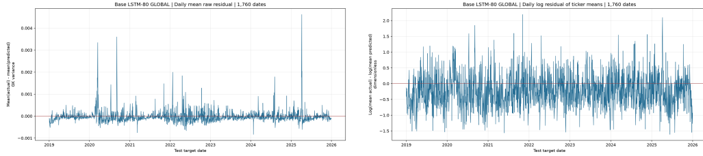
Figure 6.5: Base LSTM-80 Global: raw and log daily cross-ticker mean residual timelines (left and right).
