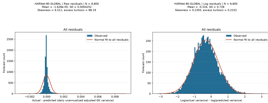
Figure 6.12: HARNet-80 Global: raw and log individual-residual histograms (left and right).
