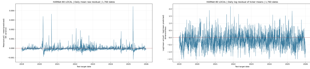
Figure 6.13: HARNet-80 Local: raw and log daily cross-ticker mean residual timelines (left and right).
