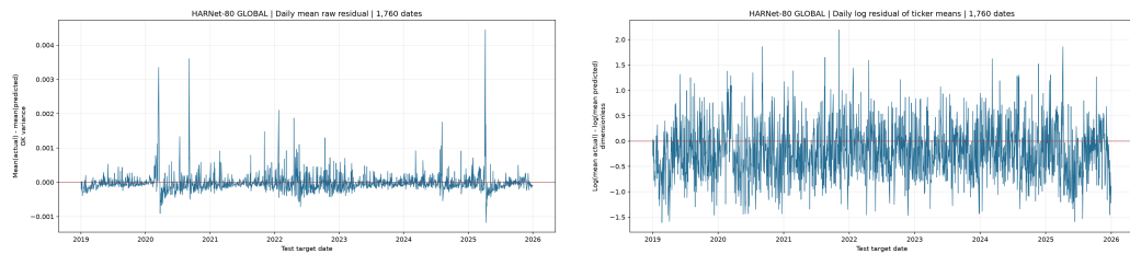
Figure 6.11: HARNet-80 Global: raw and log daily cross-ticker mean residual timelines (left and right).
