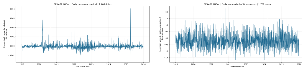
Figure 6.19: RFSV-20 Local: raw and log daily cross-ticker mean residual timelines (left and right).
