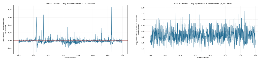
Figure 6.15: MLP-20 Global: raw and log daily cross-ticker mean residual timelines (left and right).
