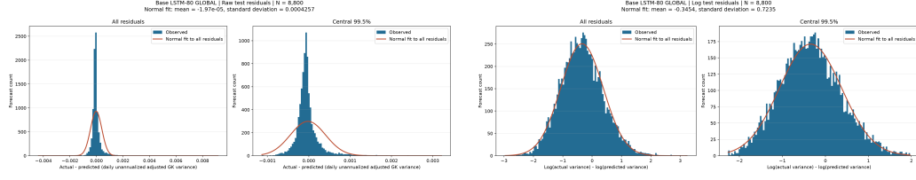
Figure 6.6: Base LSTM-80 Global: raw and log individual-residual histograms (left and right). Each histogram shows all 8,800 residuals and a display-trimmed central 99.5% panel; the orange curve is a full-sample normal fit.
