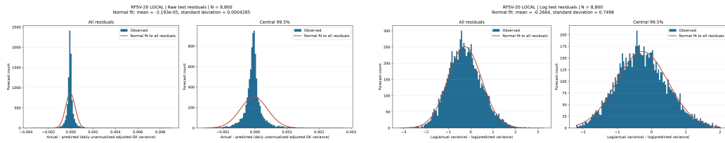
Figure 6.20: RFSV-20 Local: raw and log individual-residual histograms (left and right). Each histogram shows all 8,800 residuals and a display-trimmed central 99.5% panel; the orange curve is a full-sample normal fit.
