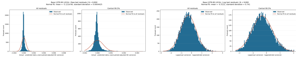
Figure 6.8: Base LSTM-80 Local: raw and log individual-residual histograms (left and right). Each histogram shows all 8,800 residuals and a display-trimmed central 99.5% panel; the orange curve is a full-sample normal fit.
