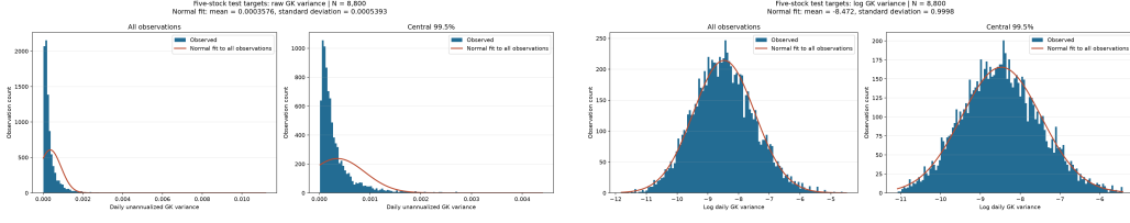
Figure 6.2: Five-stock test targets: pooled raw and log variance histograms (left and right). Each shows the full distribution and a central 99.5% display panel; the orange curve is fitted to all 8,800 targets.
