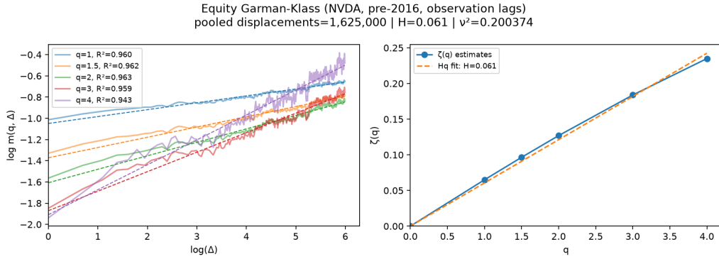
Figure A.2: Pre-2016 NVDA Garman–Klass log-volatility displacement scaling and H fit.
