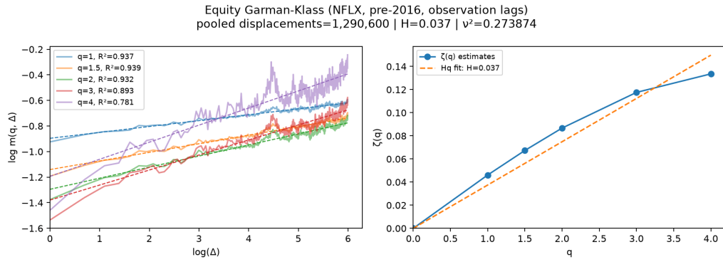
Figure A.4: Pre-2016 NFLX Garman-Klass log-volatility displacement scaling and H fit.
