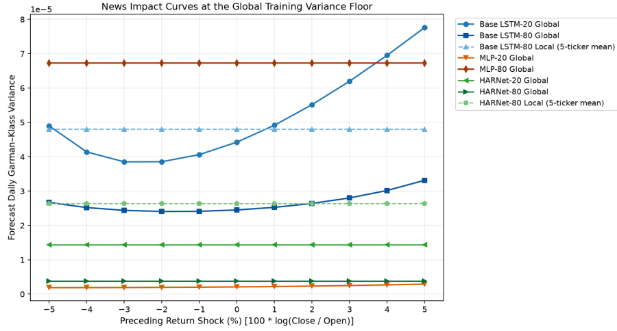
Figure 5.25: One-step forecast daily adjusted Garman–Klass variance against the synthetic signed return shock for eight MCS variants at the global training floor variance.
