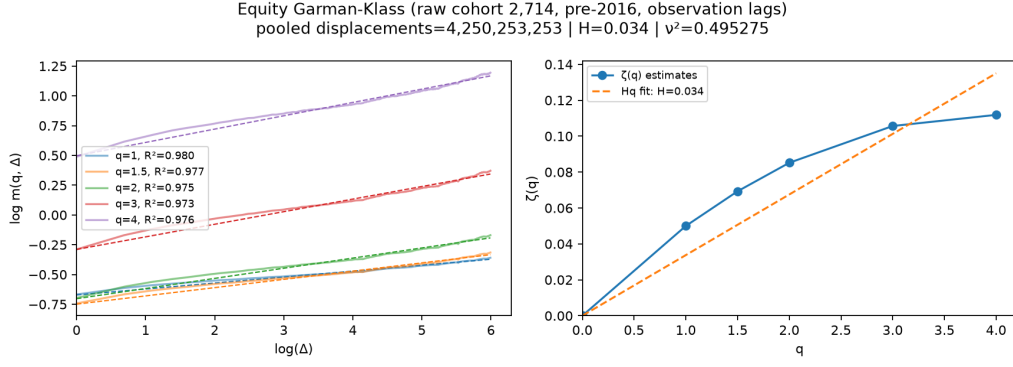
Figure A.1: Pre-2016 global Garman–Klass log-volatility displacement scaling and H fit.
