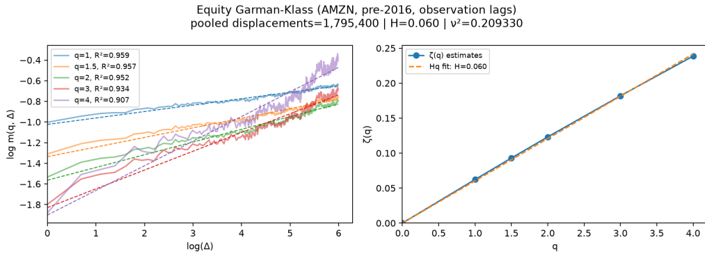
Figure A.6: Pre-2016 AMZN Garman–Klass log-volatility displacement scaling and H fit.
