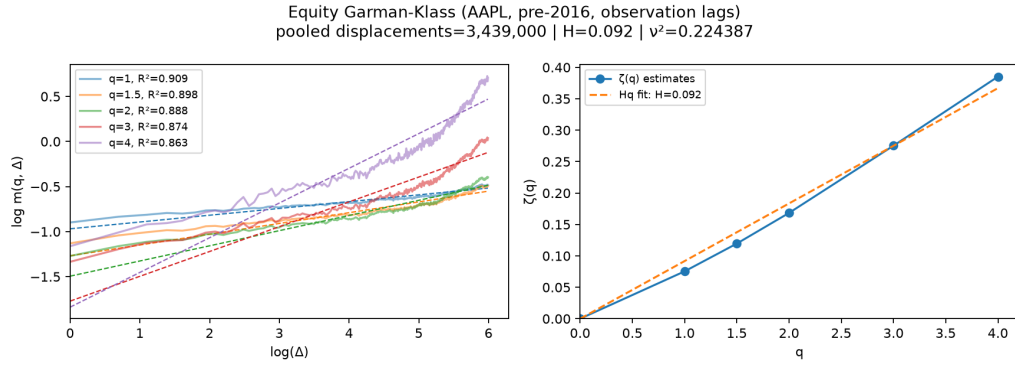
Figure A.3: Pre-2016 AAPL Garman-Klass log-volatility displacement scaling and H fit.
