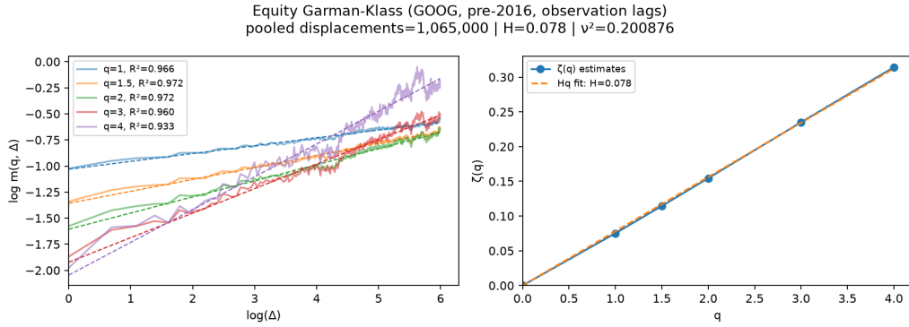
Figure A.5: Pre-2016 GOOG Garman–Klass log-volatility displacement scaling and H fit.
