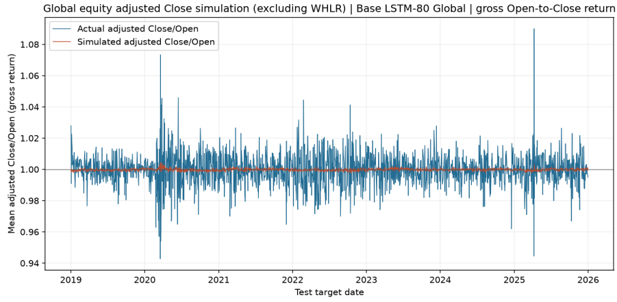
Figure 6.33: WHLR-excluded global equity daily mean adjusted Open-to-Close gross return: observed (blue) and Base LSTM-80 Global forecast-conditioned simulation (red).
