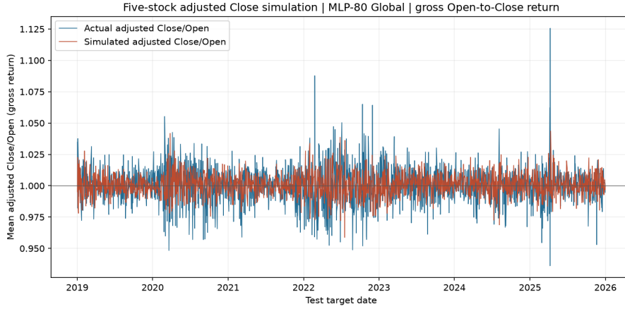
Figure 6.32: Five-stock daily mean adjusted Open-to-Close gross return: observed (blue) and MLP-80 Global forecast-conditioned simulation (red).
