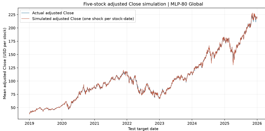
Figure 6.28: Five-stock test-date mean adjusted Close: observed (blue) and one-shock simulation using saved MLP-80 Global daily variance forecasts (red).
