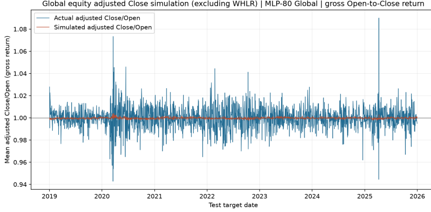
Figure 6.34: WHLR-excluded global equity daily mean adjusted Open-to-Close gross return: observed (blue) and MLP-80 Global forecast-conditioned simulation (red).
