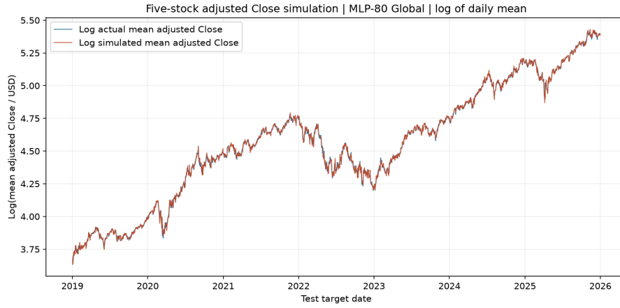
Figure 6.30: Natural log of the five-stock test-date arithmetic mean adjusted Close: observed (blue) and MLP-80 Global variance-based simulation (red).
