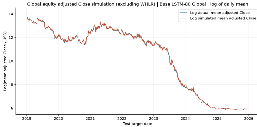
Figure 6.31: Natural log of the global equity test-date arithmetic mean adjusted Close, excluding WHLR: observed (blue) and Base LSTM-80 Global variance-based simulation (red).
