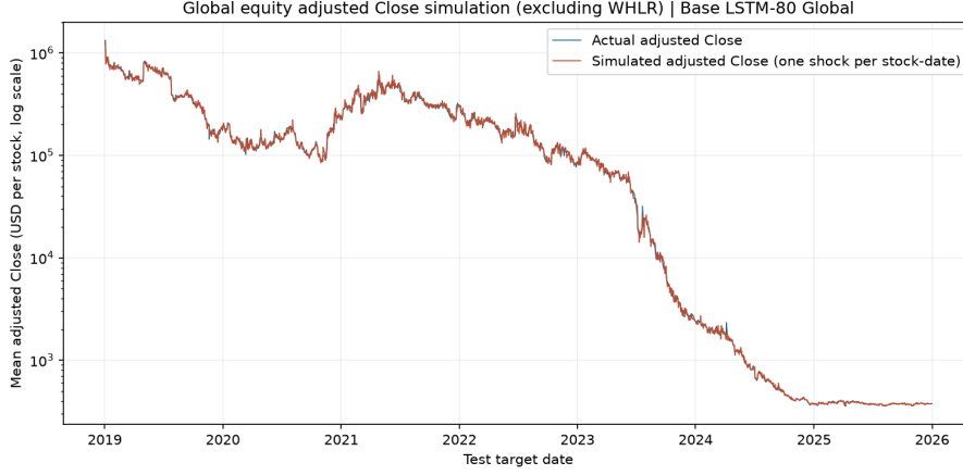
Figure 6.29: Global equity test-date mean adjusted Close, excluding WHLR, on a logarithmic vertical scale: observed (blue) and one-shock simulation using Base LSTM-80 Global daily variance forecasts (red).
