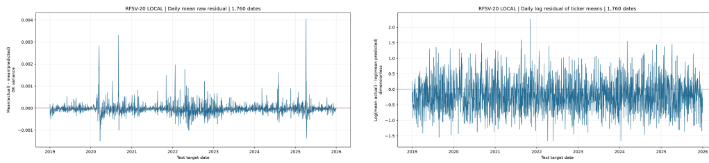
Figure 6.19: RFSV-20 Local: raw and log daily cross-ticker mean residual timelines (left and right).
