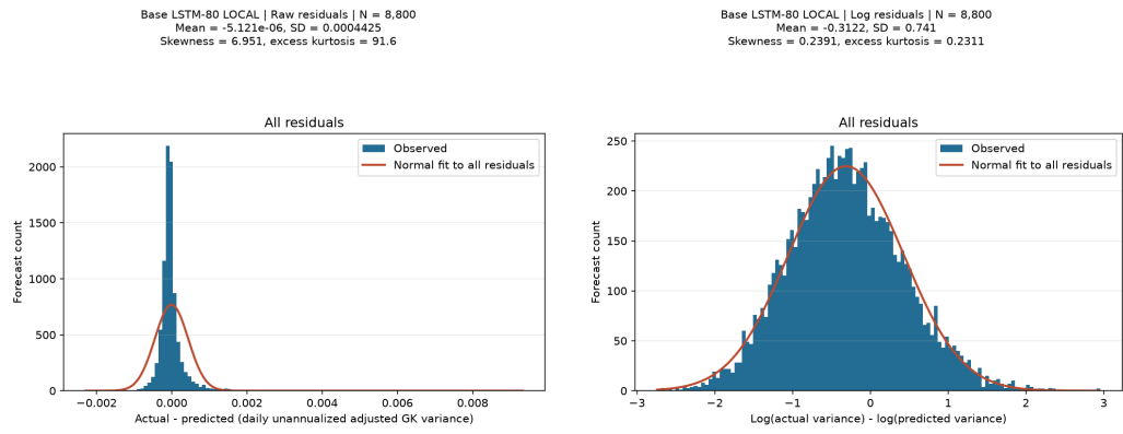
Figure 6.8: Base LSTM-80 Local: raw and log individual-residual histograms (left and right). Each histogram shows all 8,800 residuals; the orange curve is a full-sample normal fit.
