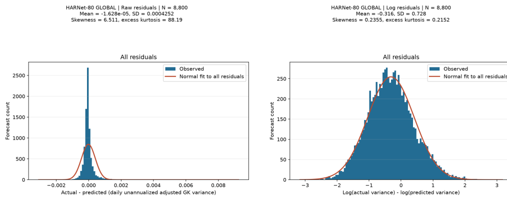
Figure 6.12: HARNet-80 Global: raw and log individual-residual histograms (left and right). Each histogram shows all 8,800 residuals; the orange curve is a full-sample normal fit.
