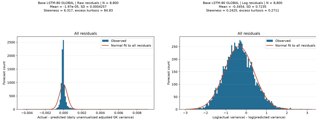
Figure 6.6: Base LSTM-80 Global: raw and log individual-residual histograms (left and right). Each histogram shows all 8,800 residuals; the orange curve is a full-sample normal fit.
