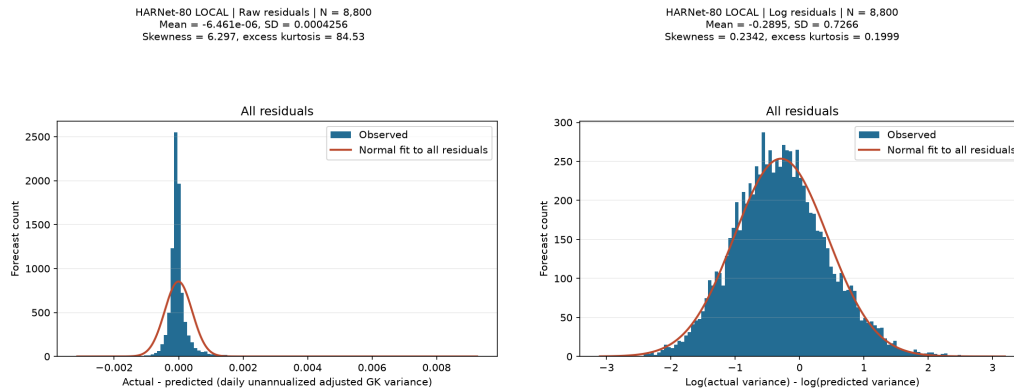
Figure 6.14: HARNet-80 Local: raw and log individual-residual histograms (left and right). Each histogram shows all 8,800 residuals; the orange curve is a full-sample normal fit.
