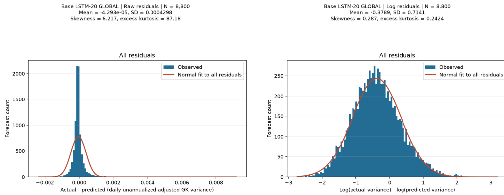
Figure 6.4: Base LSTM-20 Global: raw and log individual-residual histograms (left and right). Each histogram shows all 8,800 residuals; the orange curve is a full-sample normal fit.
