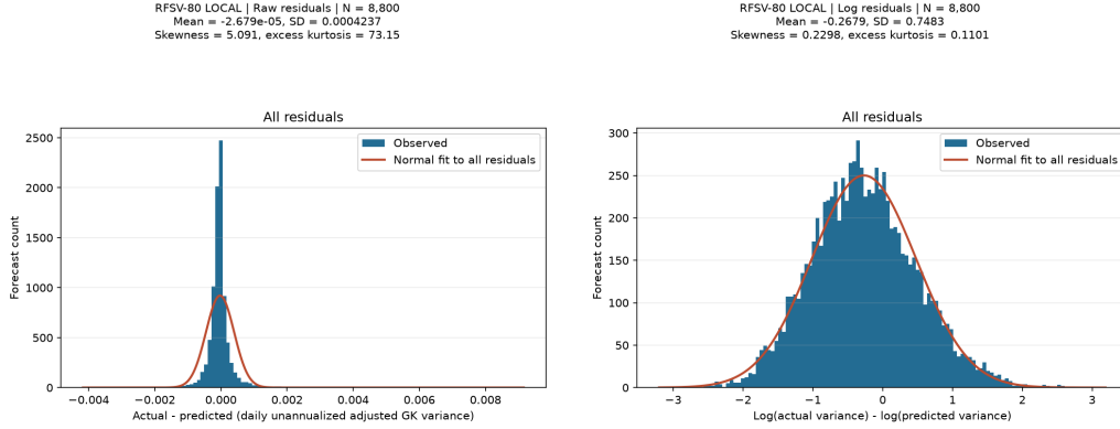
Figure 6.22: RFSV-80 Local: raw and log individual-residual histograms (left and right). Each histogram shows all 8,800 residuals; the orange curve is a full-sample normal fit.
