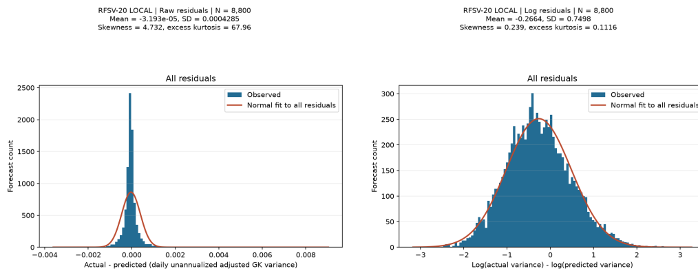
Figure 6.20: RFSV-20 Local: raw and log individual-residual histograms (left and right). Each histogram shows all 8,800 residuals; the orange curve is a full-sample normal fit.
