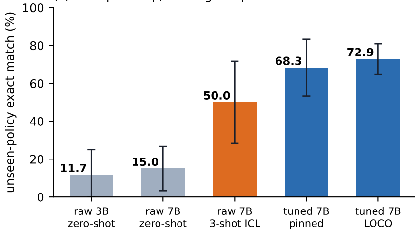
(a) Examples help, training completes
