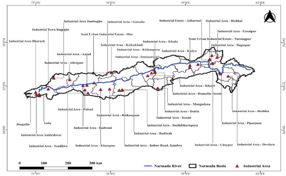
Figure 1: Spatial distribution of industrial areas across the Narmada River Basin
