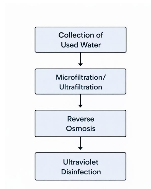
Figure 6: Steps under the NEWater treatment process
