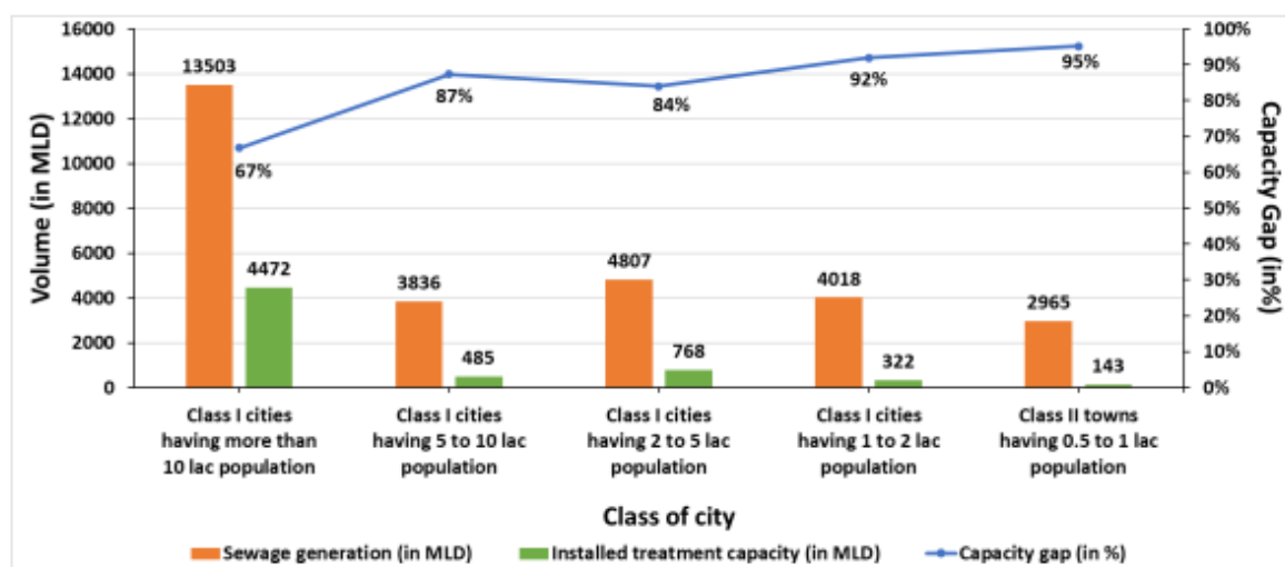
Figure 10: Wastewater generation and treatment capacity gap at the city level in India (CPCB, 2022)
