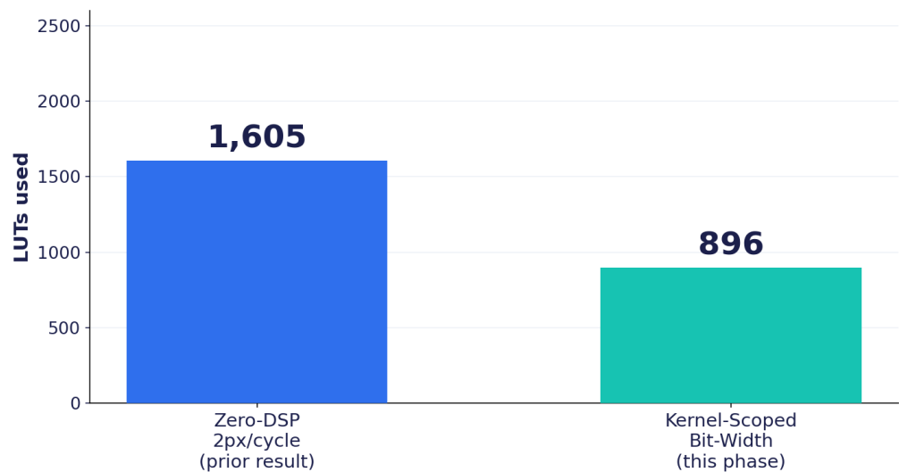
LUT Utilization Across Optimization Phases
