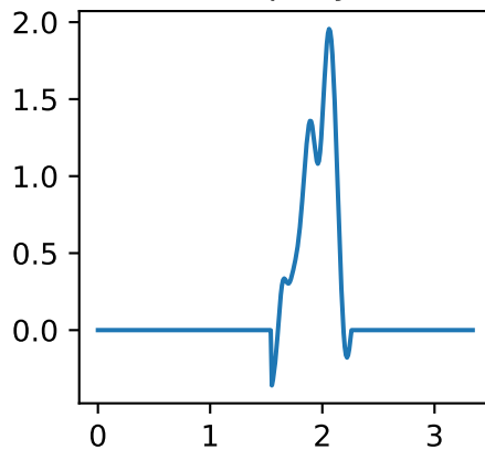
plate2 ground torque y
