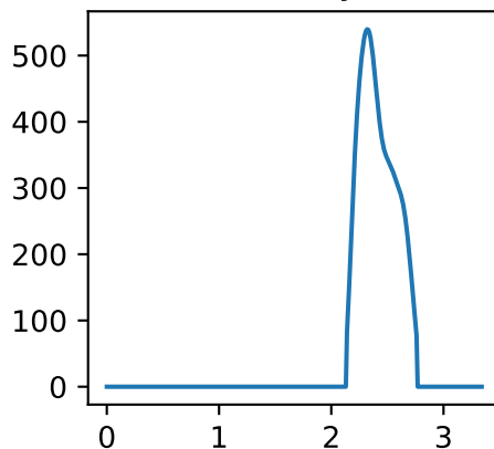
plate3 ground force py
