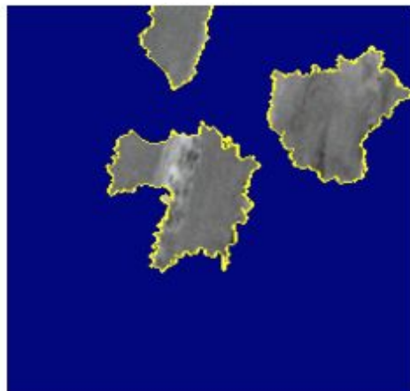
LIME: f(x)
