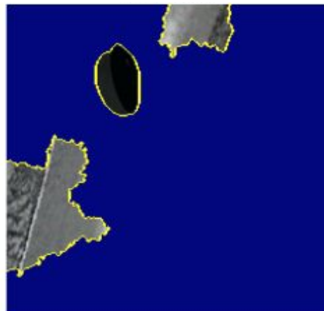
LIME: f_u(x)
