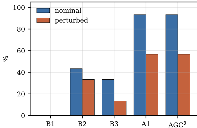
Task completion
