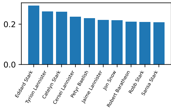
Eigenvector
