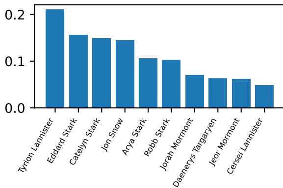
Betweenness
