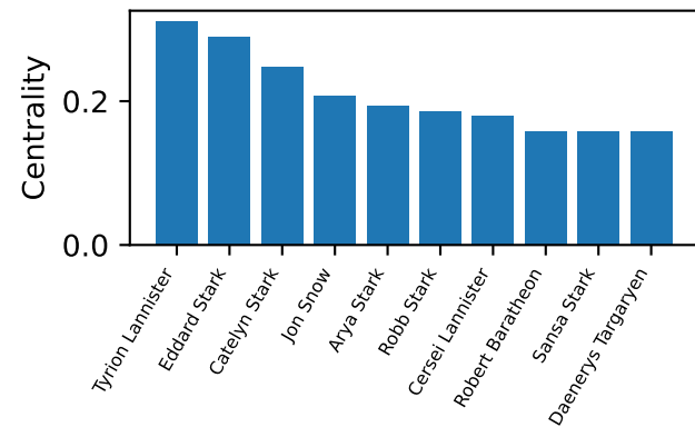
Degree
