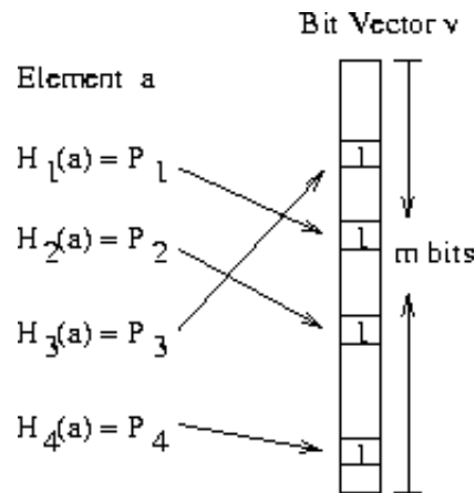
Figure 3: A Bloom Filter with 4 hash functions.
