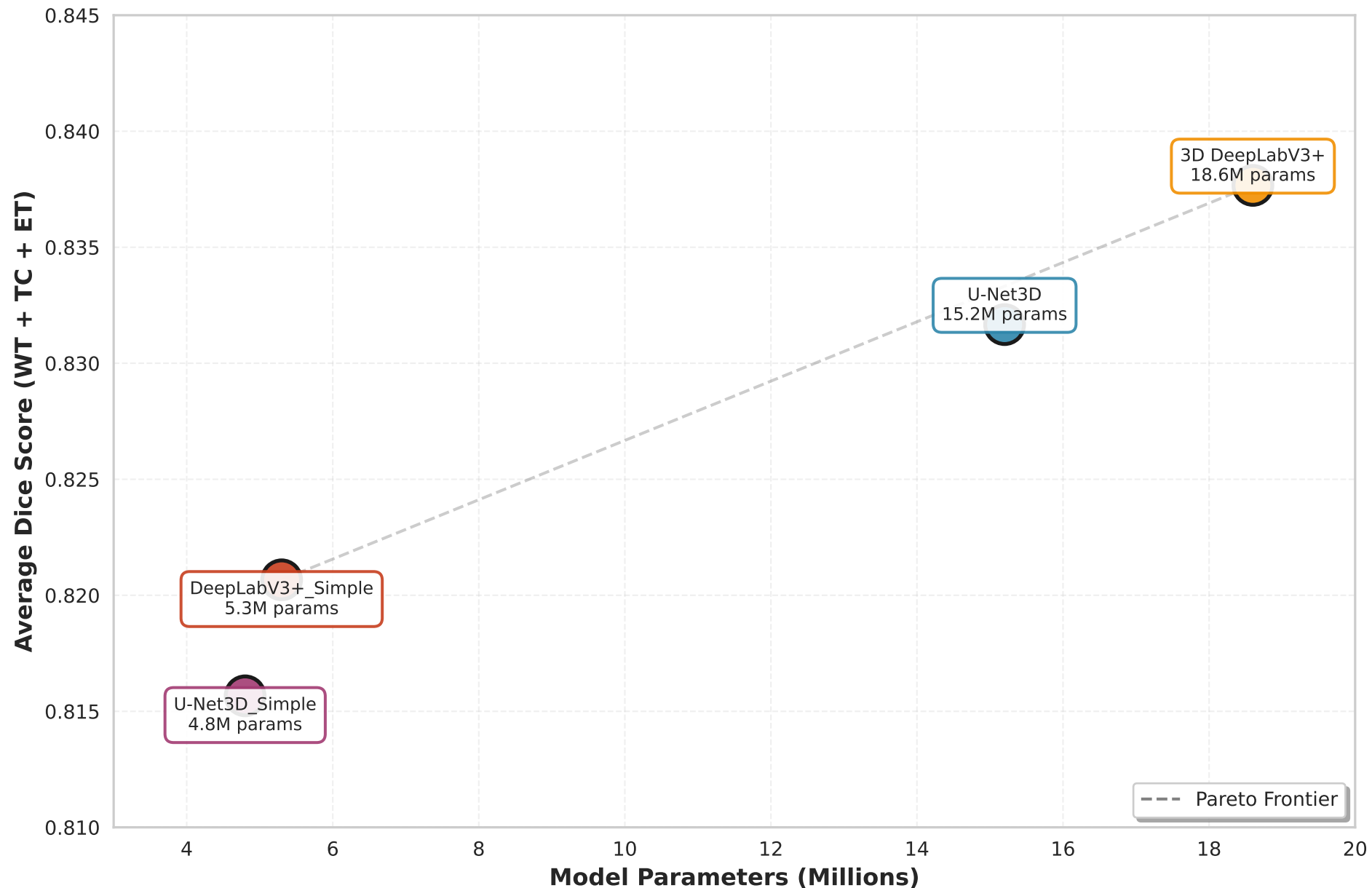
Model Performance versus Computational Efficiency
