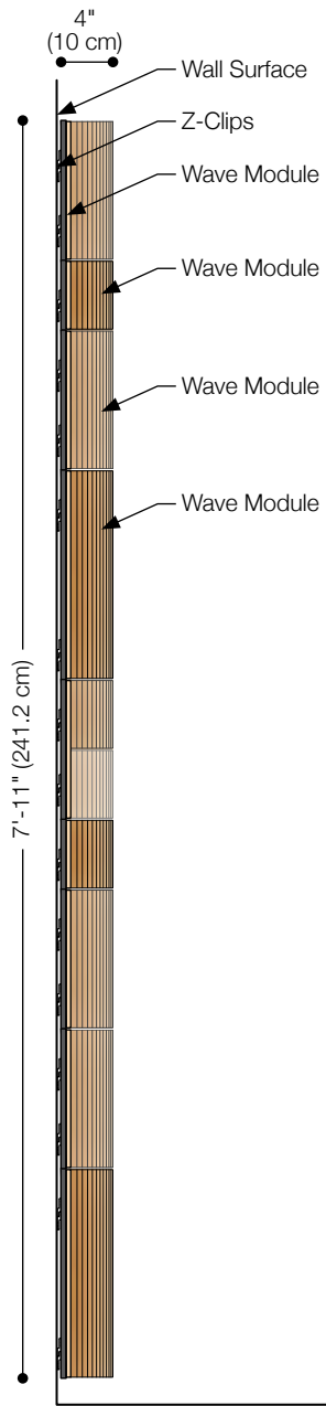
Wall Section
