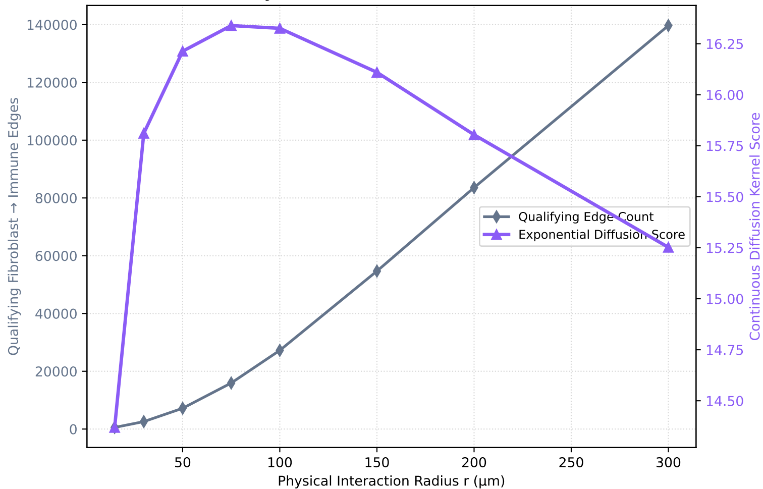
Biophysical Paracrine Scaling Connectivity Growth vs Continuous Diffusion Kernel
