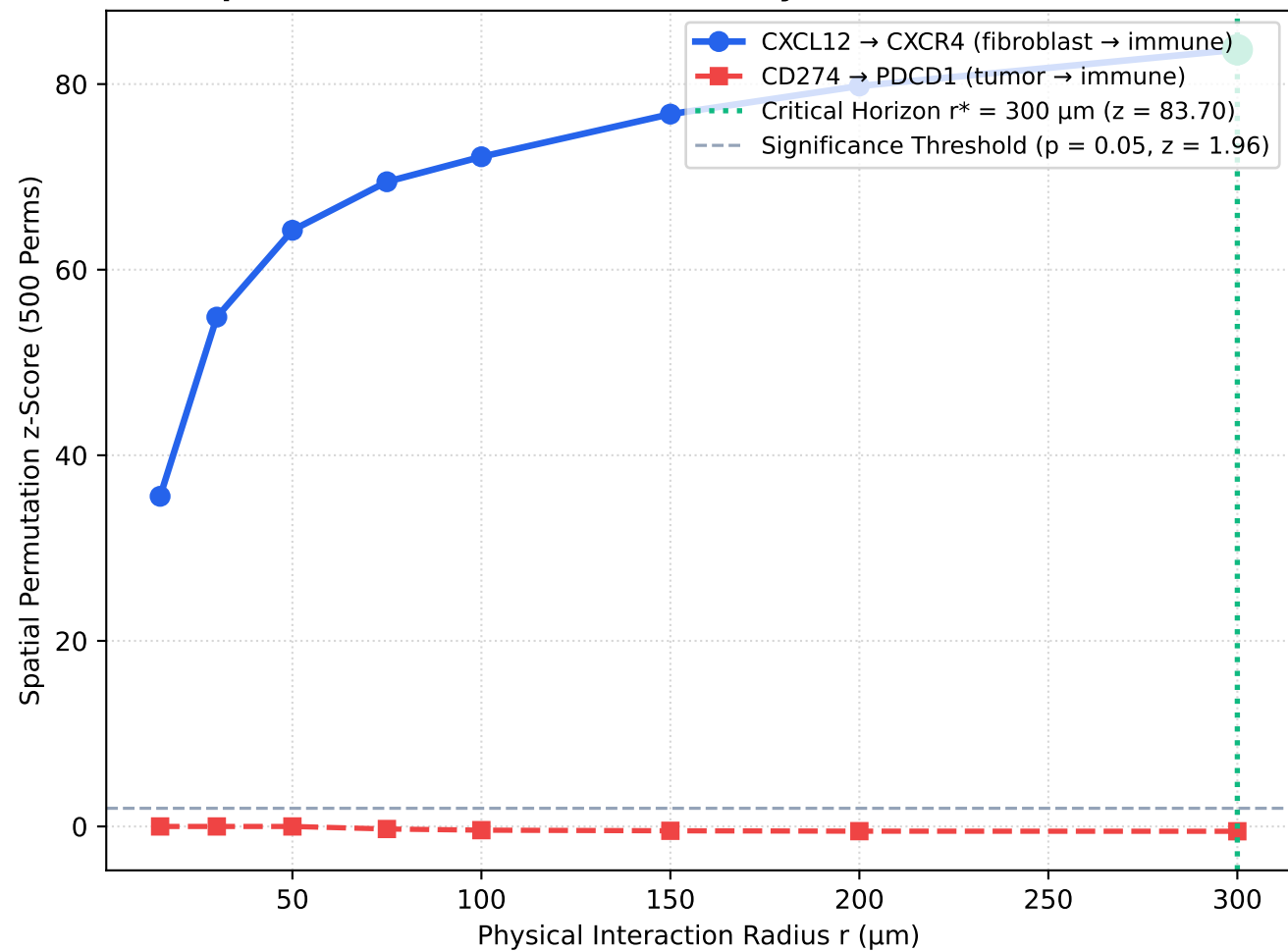
Multi-Scale Spatial Signaling Horizon Spatial Permutation z-Score vs Physical Interaction Radius
