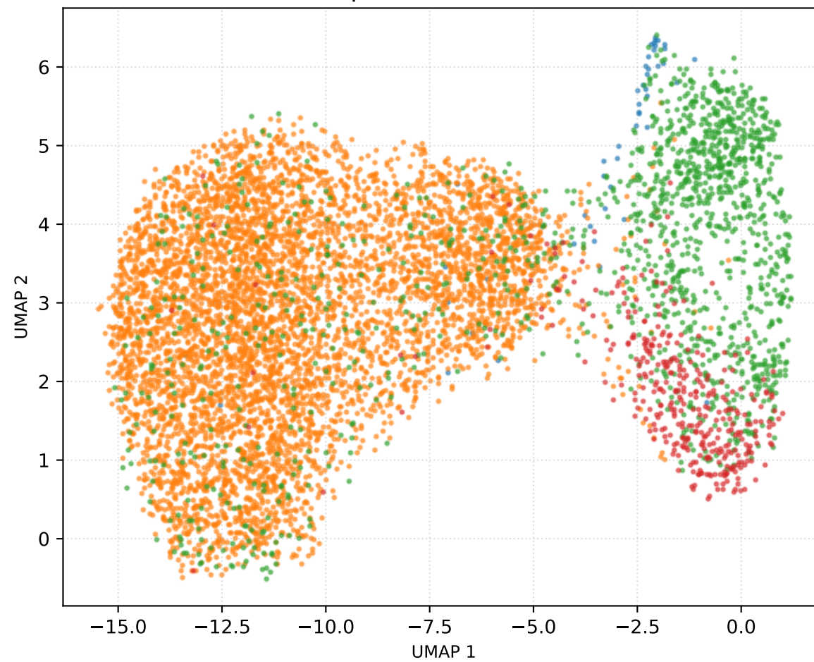
PCA-50 Baseline (Raw Expression) Silhouette: 0.1476 | Ratio vs PCA-50: 1.00 (Reference)
