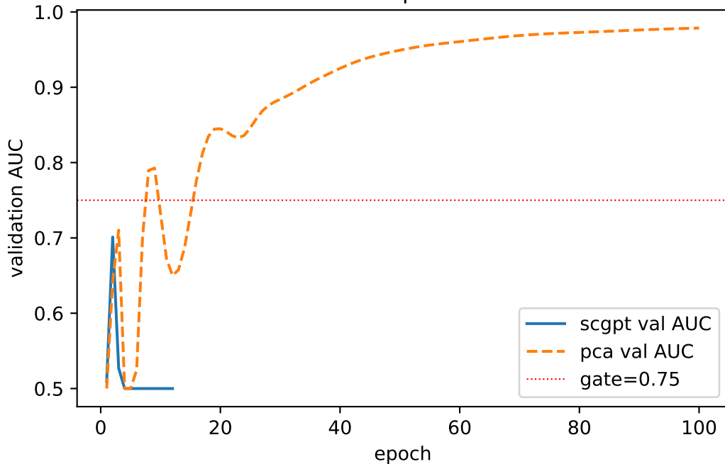
Validation link-prediction AUC
