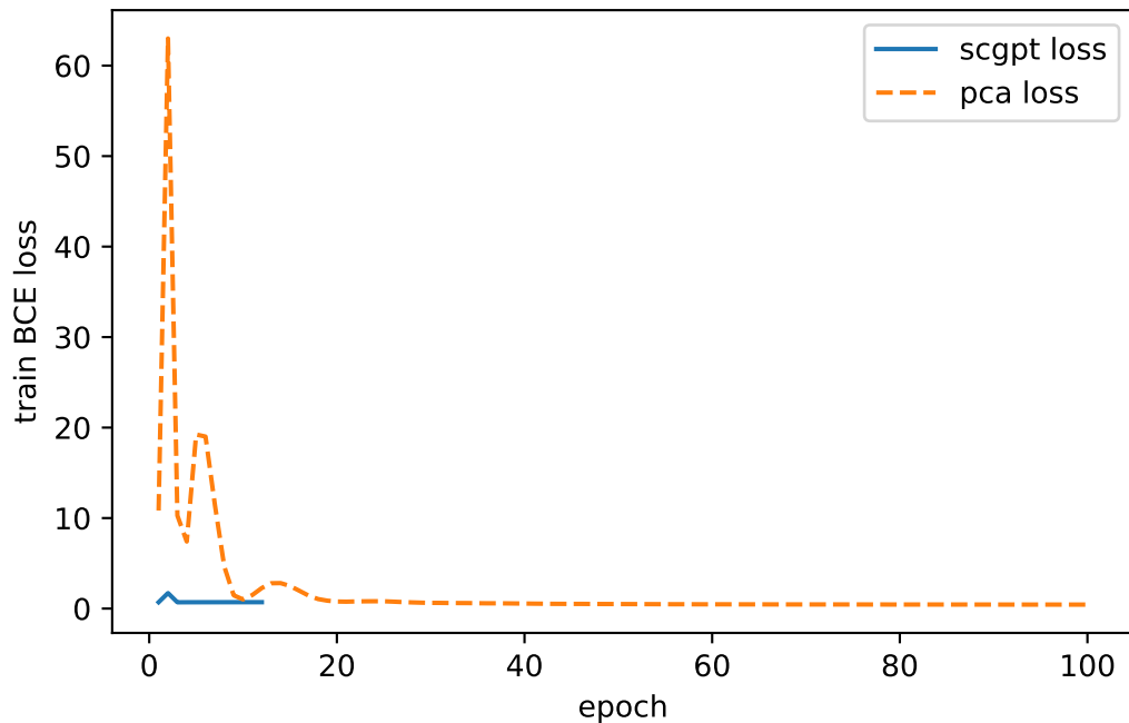
Training loss
