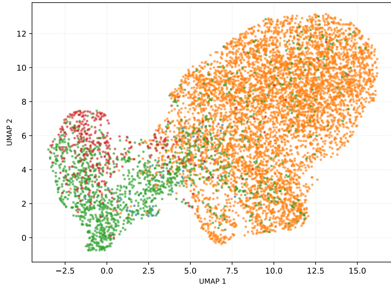
Deep Sets-50 (Permutation-Invariant) Silhouette: 0.2730 | Ratio: 1.8502
