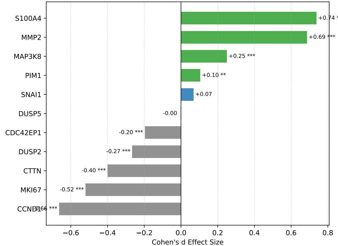
Effect Size by Gene (Engaged vs. Unengaged Receivers)
