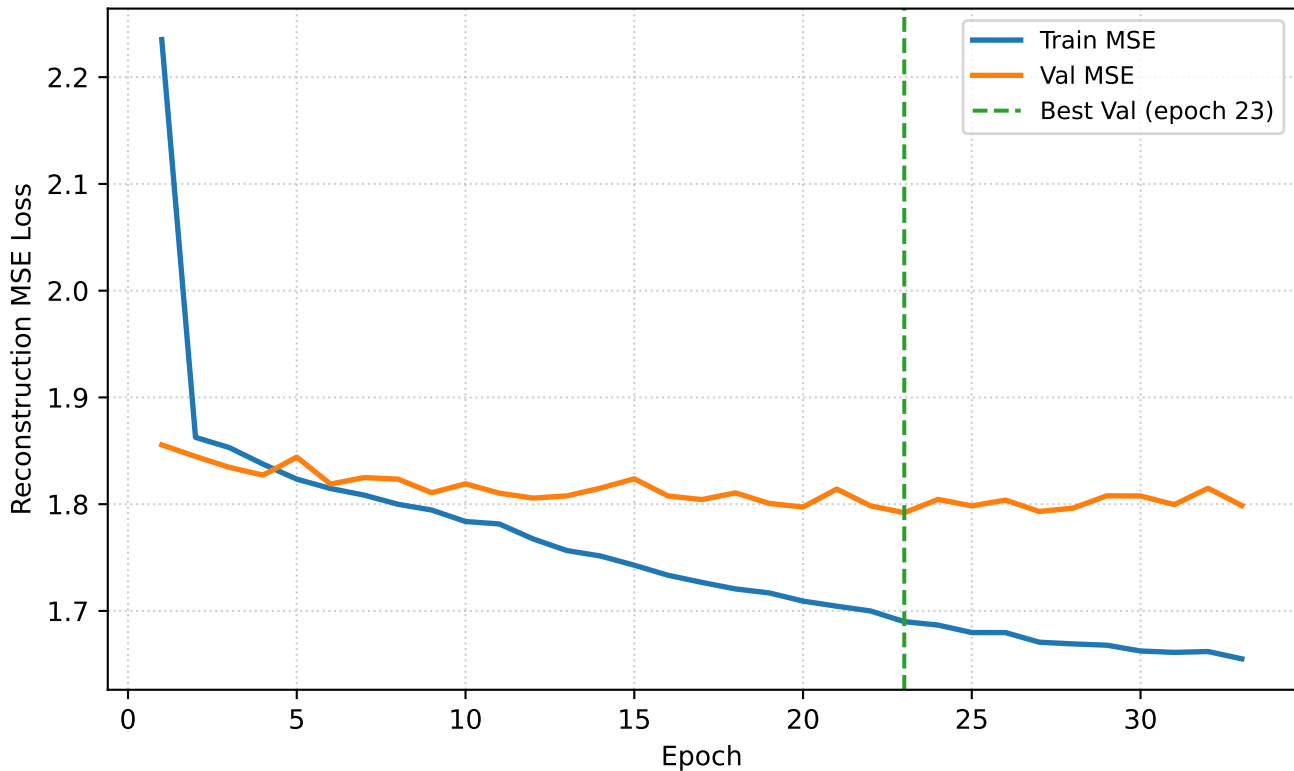
Deep Sets Spatial Feature Extractor Training Curve
