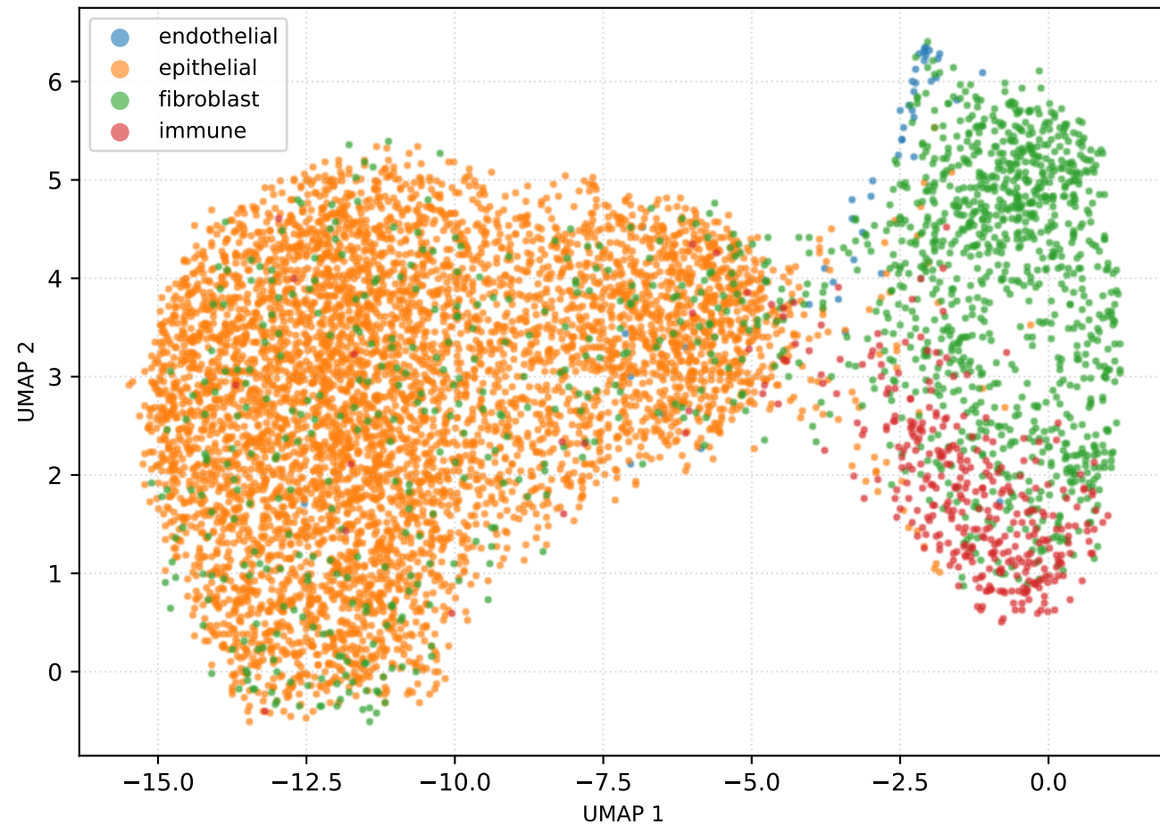
PCA-50 Baseline (Raw Expression) Silhouette: 0.1476 | Ratio vs PCA-50: 1.00 (Reference)
