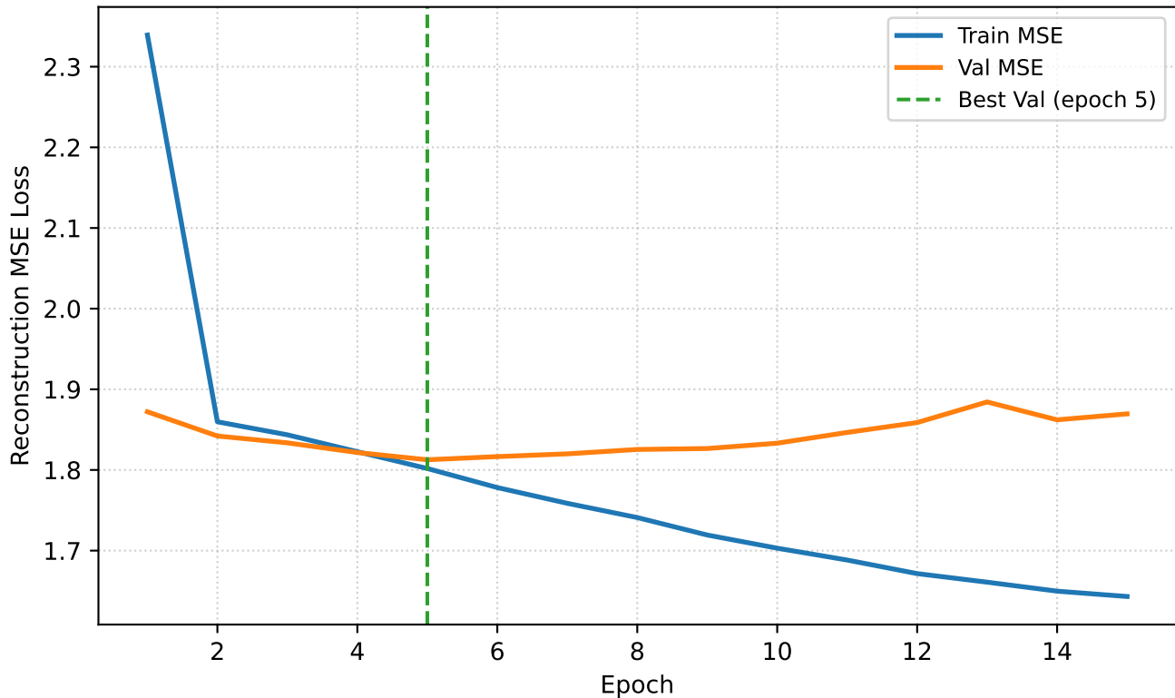
BiLSTM Spatial Feature Extractor Training Curve
