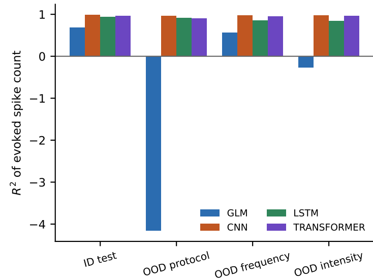
Count prediction
