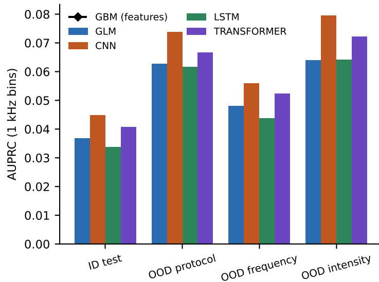
Spike detection
