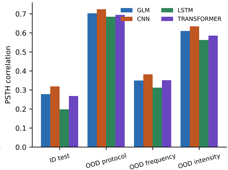
Temporal fidelity
