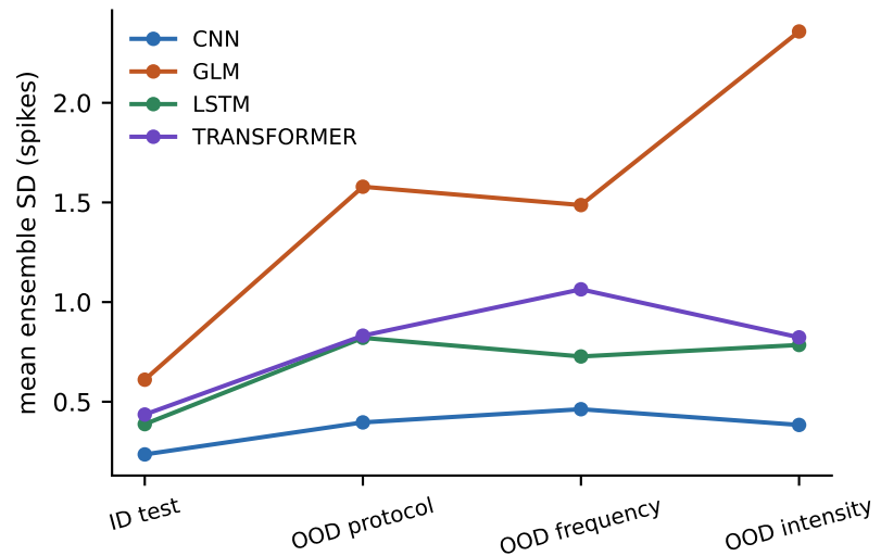
Epistemic uncertainty
