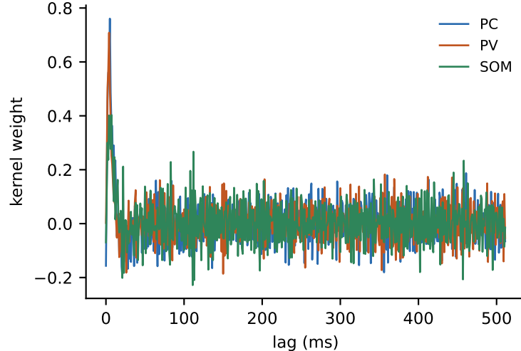
GLM impulse response by cell type
