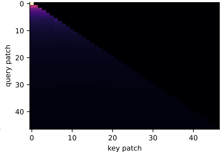
Attention (adjacent=0.17; uniform=0.23)
