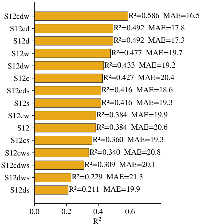
(a) Corn — R^2 by Modality
